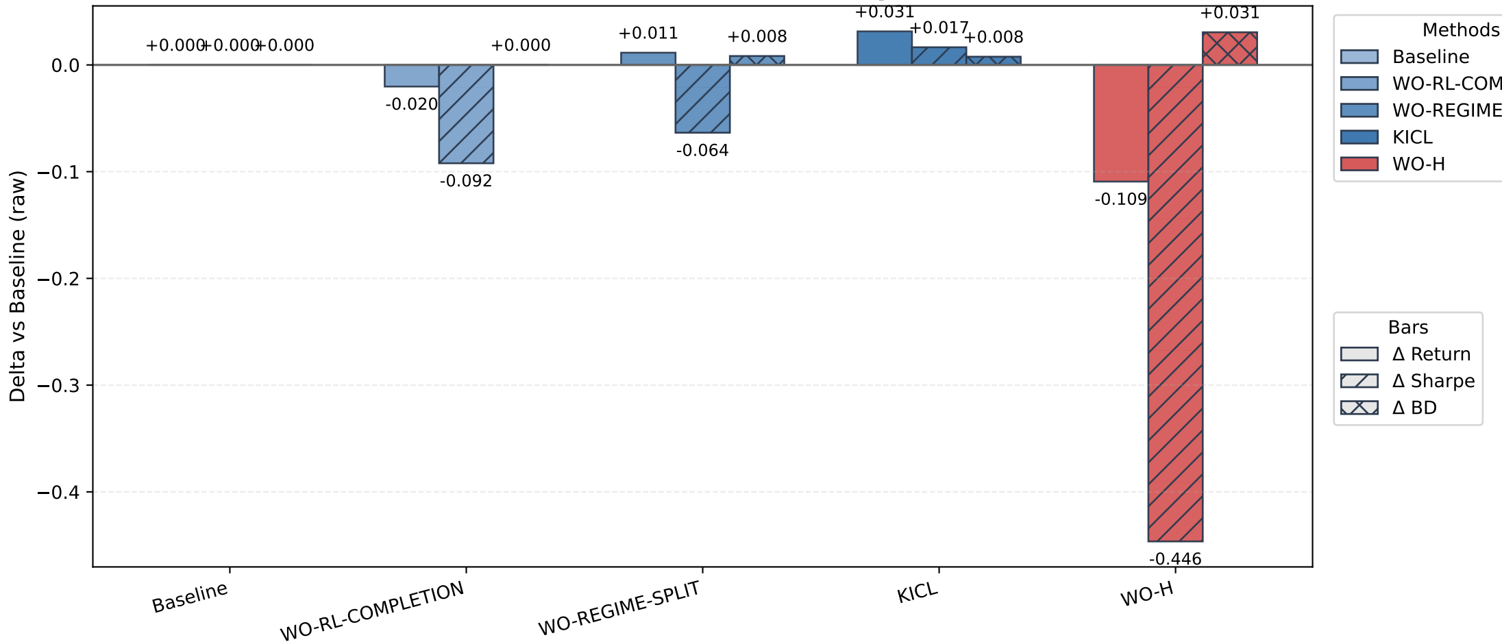
Five-Point Path: \Delta Return / \Delta Sharpe / \Delta BD
